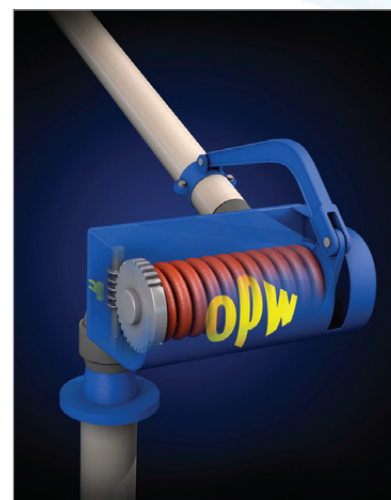
OPW Style 790 counterbalance swivel in upfeed right hand (UFRH) configuration shown.
